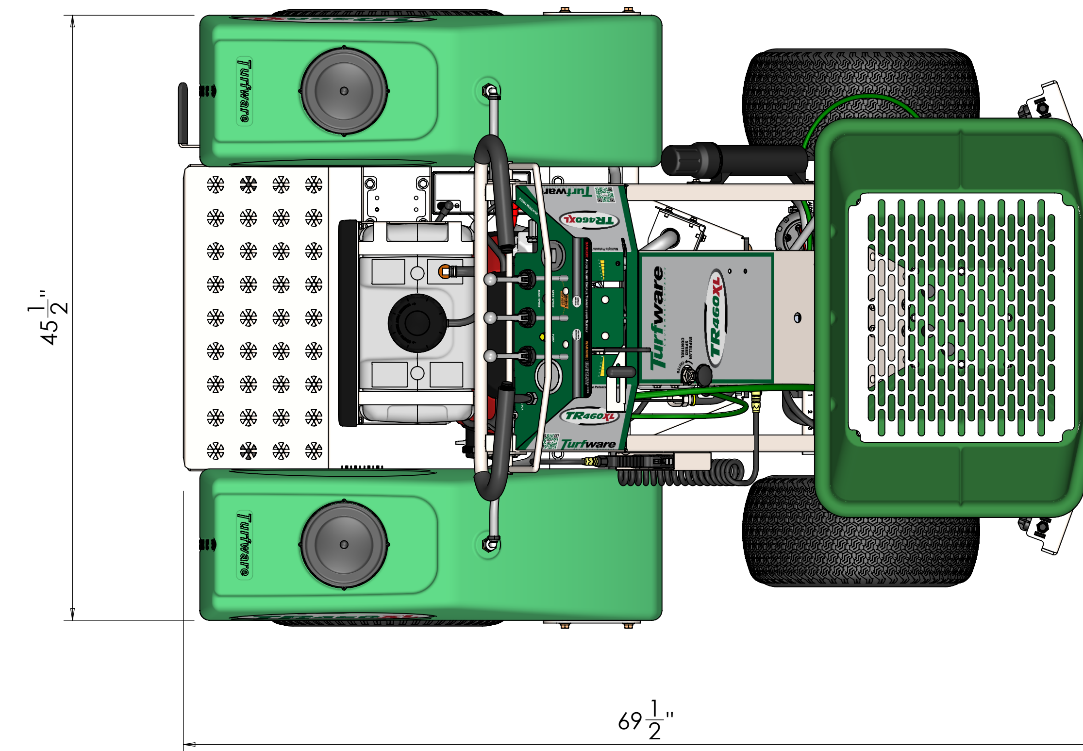
Top VIEW
