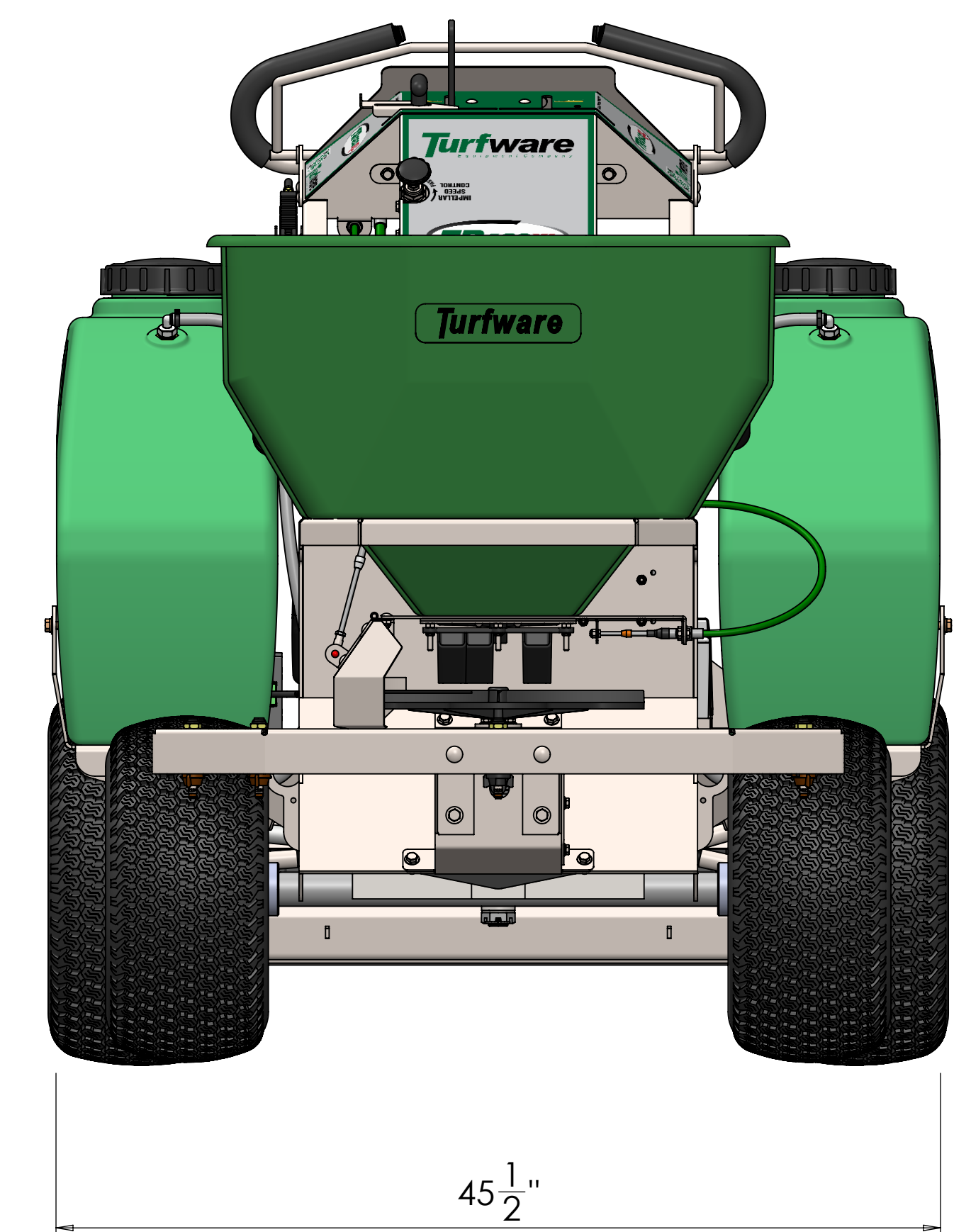
Front VIEW
