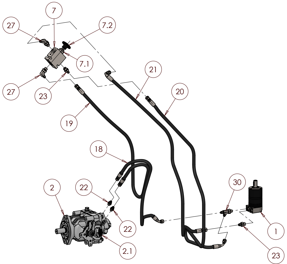
Impeller Drive Circuit
